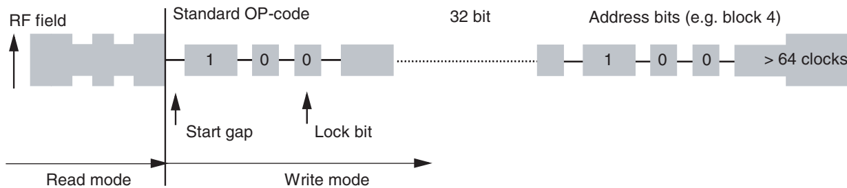
Figure 8-1. Write Protocol
